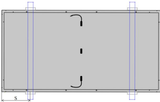
Installation of framed module with fixtures on long sides (Beam perpendicular to long sides)
