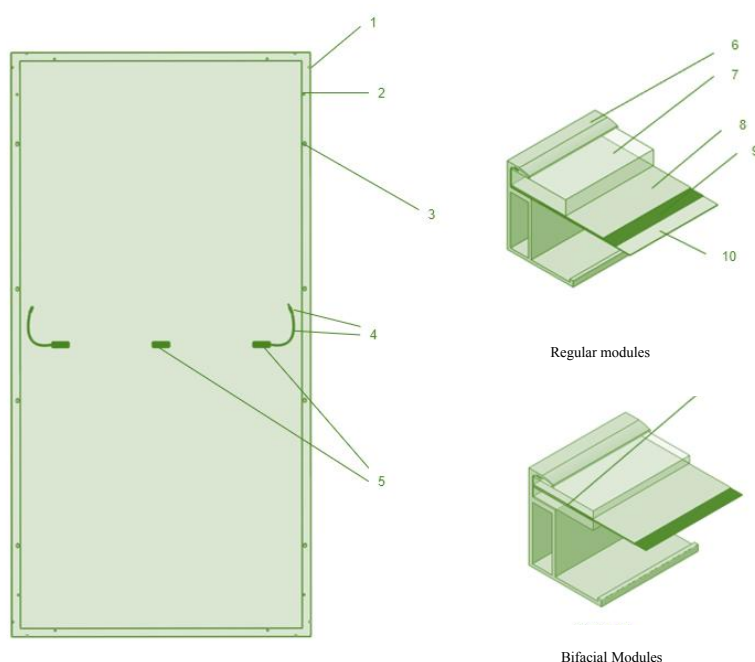
Figure 1 Regular Modules Mechanical Drawing
