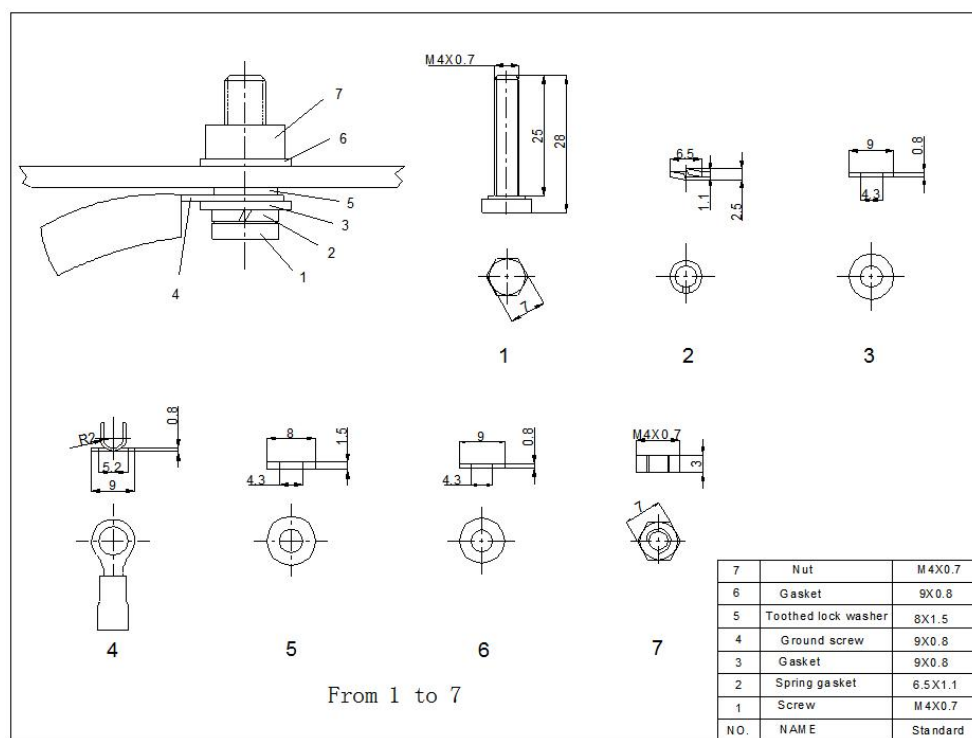
Figure 5. Example of acceptable ground connection
