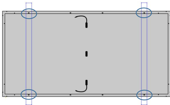
Installation with bolts into 4 outer holes (Beam perpendicular to long sides)
