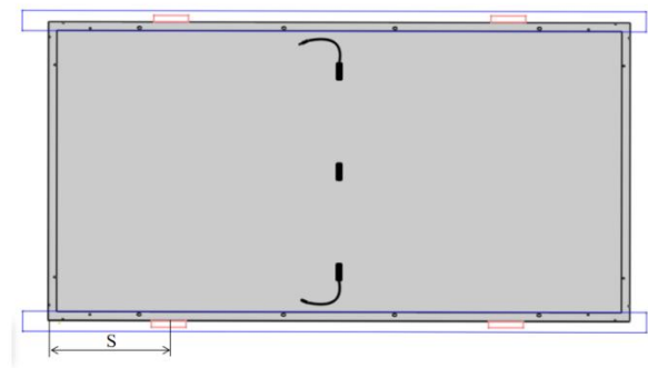
Installation of framed module with fixtures on long sides (Beam Parallel to long sides)
